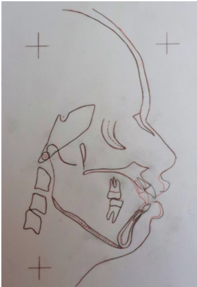
Figure 8: Cephalometric superimposition.
