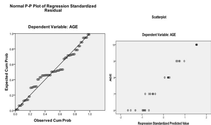
Figure 2 & 3: Plots of expected cum probability against observed cum probability, and age against regression standardized predicted value respectively.
