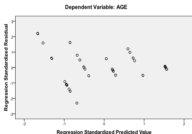
Figure4: Plots of regression standardized residuals against regression standardized predicted value.
