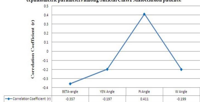
Graph 2: Correlation Coefficient of ANB angle with various new cephalometric parameters among Skeletal Class I Malocclusion patients.
